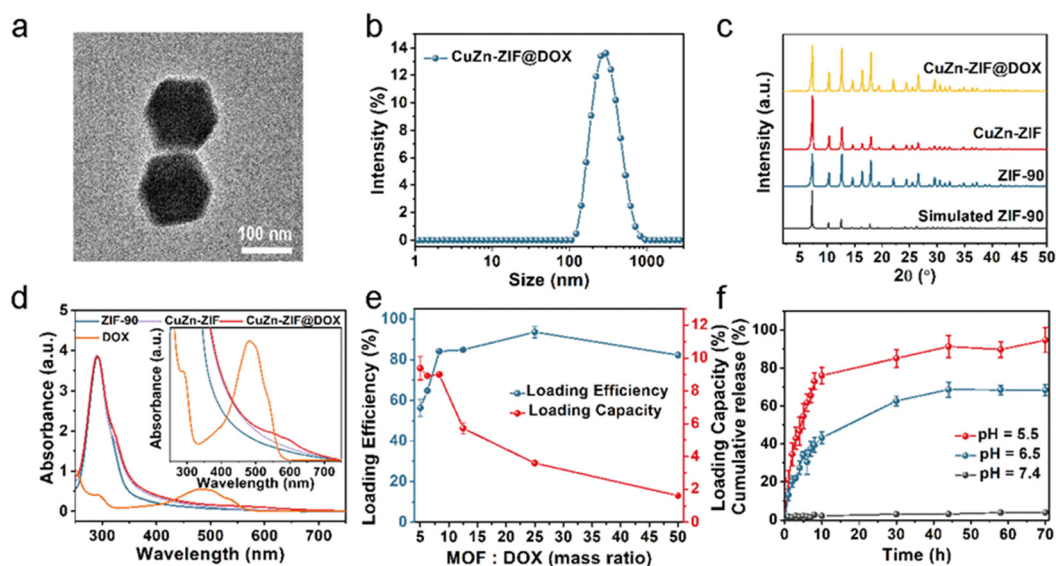
Fig. 3 (a) TEM image of CuZn-ZIF@DOX. (b) Size distribution of CuZn-ZIF@DOX. (c) PXRD patterns of CuZn-ZIF@DOX. (d) UV-vis spectra of ZIF-90, CuZn-ZIF, CuZn-ZIF@DOX, and DOX (inset: the enlarged figure). (e) The loading efficiency and loading capacity of DOX to CuZn-ZIF at a series of mass ratios. (f) The release of DOX from CuZn-ZIF@DOX at different pH values.
