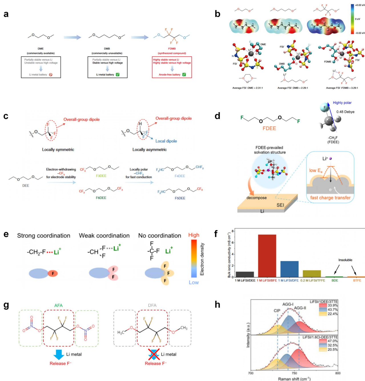
Fig. 8 (a) Design scheme and molecular structures of three liquids: DME, DMB and solvation structure of 1 M LiFSI/DME, 1 M LiFSI/DMB and 1 M LiFSI/FDMB. Reproduced with permission. Copyright © 2020, Nature Publishing Group. (c) Logical flow, starting from DEE, for the design of the fluorinated-DEE family. Spatial configuration and dipole direction of -\text{CF}_3 and -\text{CHF}_2 . Reproduced with permission. Copyright © 2022, Nature Publishing Group. (d) Illustration of FDEE-prevalent solvation structure forming the SEI with facilitated \text{Li}^+ transport. Reproduced with permission. Copyright © 2023 American Chemical Society. (e) Coordination chemistry of monofluoro, difluoro, and trifluoro groups. (f) Bulk ionic conductivities of various electrolytes at 30 °C, including DEE, BTFE, BDE, TFFE, DFE, and BFE. Reproduced with permission. Copyright © 2023, Nature Publishing Group. (g) Molecular design of AFA with active nitrate ending group and DFA with inert methoxyl on the side of fluorocarbon segment. Reproduced with permission. Copyright © 2022 WILEY-VCH. (h) Raman spectra and the population of AGGs-II (red, 755 \text{cm}^{-1} ), AGGs-I (blue, 744 \text{cm}^{-1} ), and CIPs (yellow, 731 \text{cm}^{-1} ) in the two electrolyte systems. Reproduced with permission. Copyright © 2022 WILEY-VCH.
