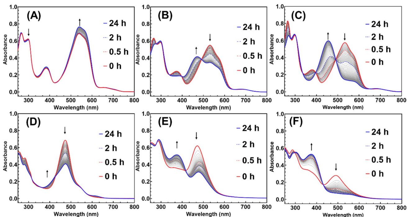
Fig. 2 The spectral evolution of \text{Et}_2\text{N}-\text{FlavP}_1 ( 0.1 \text{ g L}^{-1} ) at 25^\circ\text{C} in (A) methanol; (B) deionised water and (C) universal buffer (pH 7). The spectral evolution of \text{MeO}-\text{FlavP}_1 ( 0.1 \text{ g L}^{-1} ) at 25^\circ\text{C} in (D) methanol; (E) deionised water and (F) universal buffer (pH 7).
