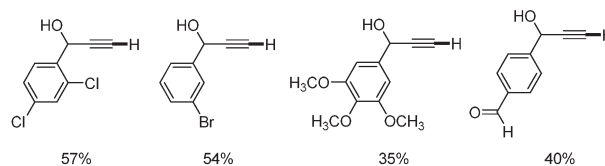
Scheme 53 Decarboxylation using \text{Pd}(\text{OH})_2/\text{C} .
