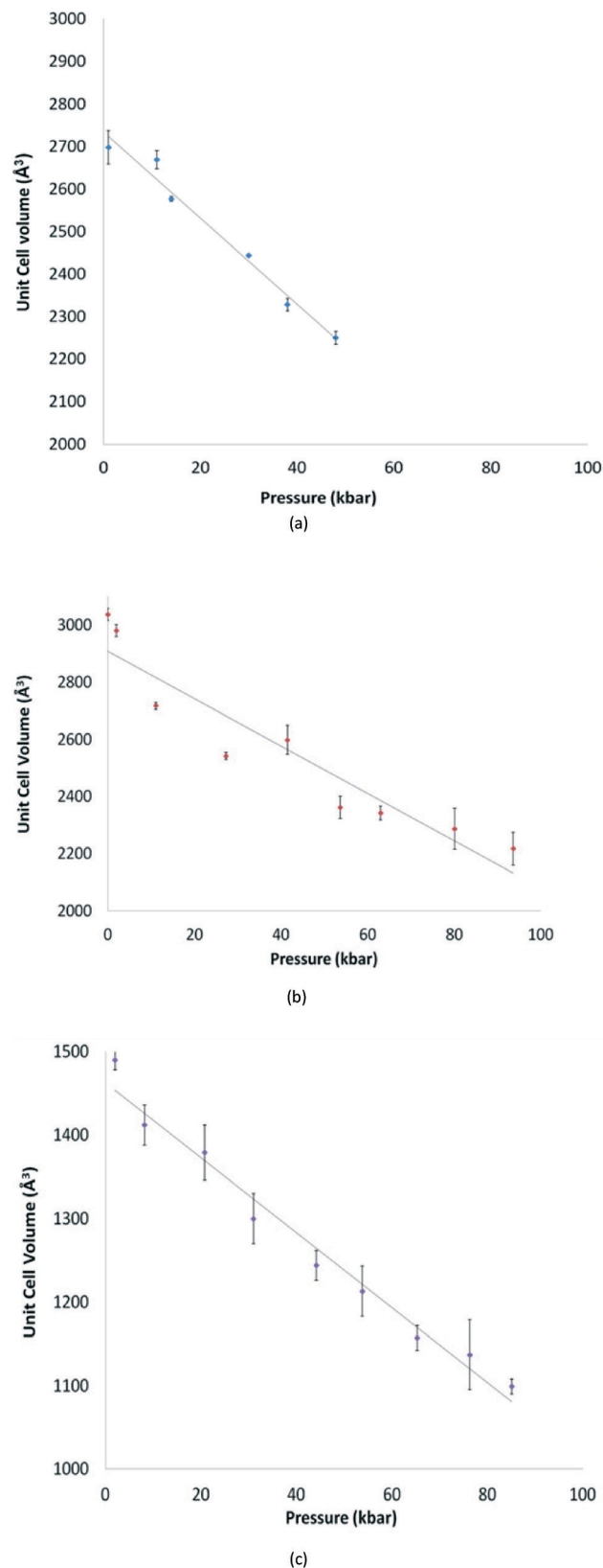
Fig. 4 Unit cell volume (Å 3 ) vs. pressure (kbar) for 1 (a, blue), 2 (b, red) and 3 (c, purple). Error bars indicate 3σ limits. Pressure values are an average of measurements taken before and after the data collection. The solid line is a guide to the eye.
