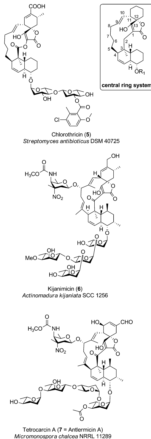
Fig. 6 Medium-sized spirotreronates. The central ring system, present in the CHL/KIJ/TCA (chlorothricin/kijanimicin/tetrocarcin A) – family comprises a central 13-membered macrocycle (carbon numbering see upper right).
