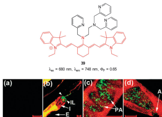
Fig. 34 Top: cyanine based ligand 39 . Bottom: imaging of cyanide in C. elegans infected with P. aeruginosa (GFP). Prior to incubation with 39-Cu(II) . C. elegans nematodes were fed for 2 d on non-infectious E. coli OP50 (a) or GFP-labelled PA14 (b–d). (b) the anterior end, (c) the medial part, (d) the posterior. (I = intestine; IL = intestinal lumen; I = intestine; E = eggs; PA = PA14-GFP; A = anus). Scale = 20 \mu m. Image reproduced with permission. 181
