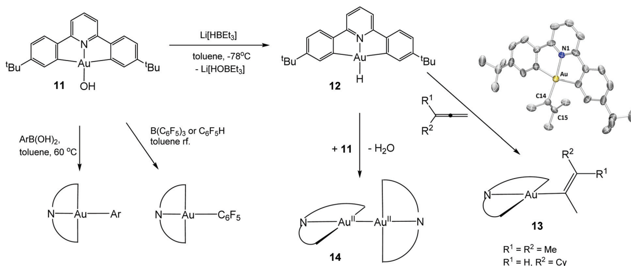
Scheme 8 Formation and reactivity of (C ^ N ^ C)Au(III)H.
