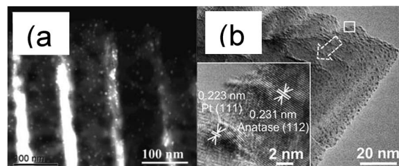
Fig. 24 (a) Dark field (S)TEM image of ultrafine Pt NPs deposited on TiO 2 nanotube arrays, 220 and (b) TEM image of size-resolved ultrafine Pt NPs on TiO 2 film. Inset: HRTEM image showing the lattice fringes corresponding to anatase TiO 2 (112) and Pt (111) NPs. Reproduced from ref. 157 with permission from The Royal Society of Chemistry.
