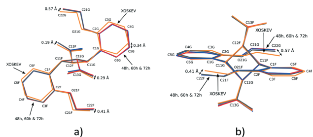
Fig. 9 Two different views of the superimposition of FG photodimer molecules from XOSKEV (recrystallized photodimer), 48, 60 and 72 h.
