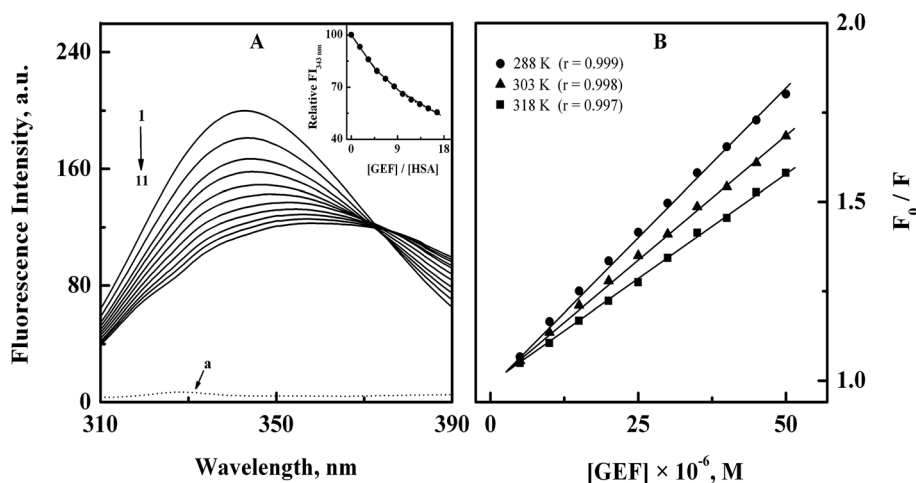
Fig. 2 (A) Fluorescence quenching spectra of 3 \text{ \mu M} HSA (spectrum 1) with increasing concentrations ( 5 – 50 \text{ \mu M} with 5 \text{ \mu M} intervals) of GEF (spectra 2–11), obtained in 60 \text{ mM} sodium phosphate buffer, \text{pH } 7.4 at 15 \text{ }^\circ\text{C} upon excitation at 295 \text{ nm} . The dotted line at the bottom (a) shows the fluorescence spectrum of GEF alone. Inset displays the decrease in the relative fluorescence intensity of HSA at 343 \text{ nm} ( F_{343 \text{ nm}} ) with increasing GEF/HSA molar ratios. (B) Stern–Volmer plots for the binding of GEF to HSA, obtained at three different temperatures, i.e. , 288, 303 and 318 \text{ K} .
