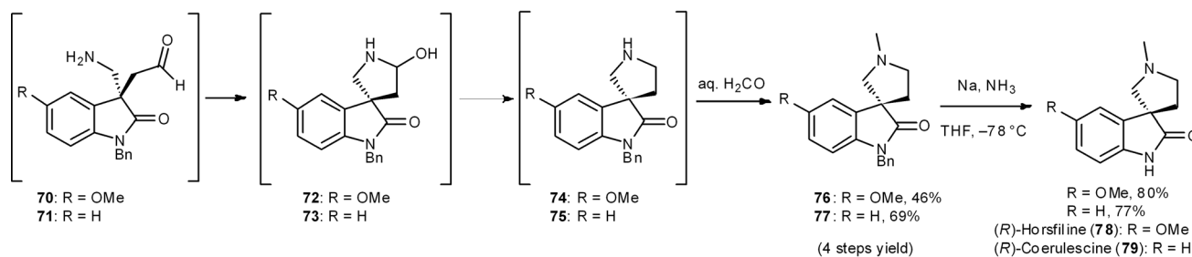
Scheme 7 Three-pot synthesis of ( R )-horsfiline and ( R )-coerulescine.
