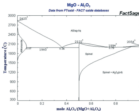
Fig. 14 Phase diagram of magnesium aluminates.
