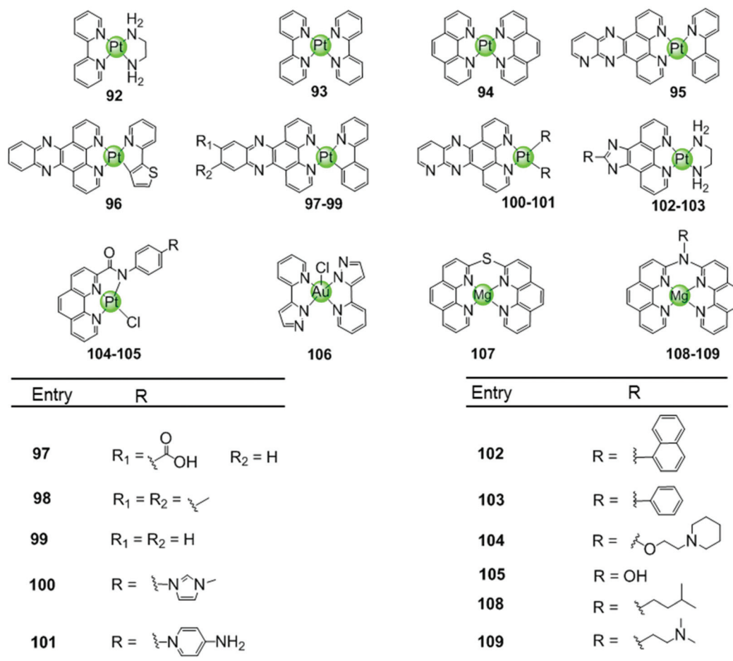
Fig. 10 Metal–phenanthroline complexes and derivatives reported as G4-ligands. The bidentate ligands are, e.g. ethylenediamine (dien), bipyridine (bpy), phenanthroline (phen), dipyriddyphenazine (dppz), phenanthroimidazol, phenylpyridine (ppy). Several Pt(II) complexes are also luminescent G4-ligands. 76–84
