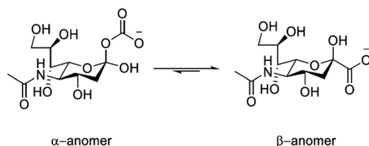
Fig. 1 Structure of sialic acid (Neu-5-Ac) showing the \alpha - and \beta -pyranose forms; \text{pK}_a = 2.6 ( \text{H}_2\text{O} , I = 0.1 , 298 K).
