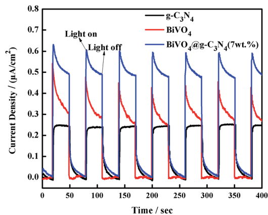
Fig. 11 Transient photocurrent response for g\text{-C}_3\text{N}_4 , \text{BiVO}_4 and \text{BiVO}_4@g\text{-C}_3\text{N}_4 photo-catalysts.
