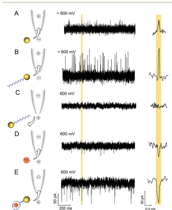
Fig. 2 Current–time traces of (A) AuNPs and (B) AuNP-LBA at –600 mV and (C) AuNP-LBA, (D) free lysozyme, and (E) AuNP-LBA/lysozyme complexes at 600 mV with 100 mM KCl. The baseline current was –1230 pA for (A) AuNPs and –1200 pA for (B) AuNP-LBA at –600 mV; 2200 pA for (D) free lysozyme and 2300 pA for (E) AuNP-LBA/lysozyme complexes at 600 mV. AuNPs and AuNP-LBA exhibited current enhancement at negative voltages (events reversed for easier interpretation) while free lysozyme and AuNP-LBA/lysozyme complexes exhibited current blockade at positive voltages. Representative individual events are shown on the right-hand side of each trace.
