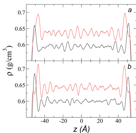
Fig. 2 Density profiles for each of the components of the ionic liquid [bmim][triflate] at a temperature of 373.15 K and at r_{ci} values of (a) 10.5 \text{ \AA} and (b) 30.5 \text{ \AA} . Black and red lines represent the [bmim] and [triflate] ions, respectively.
