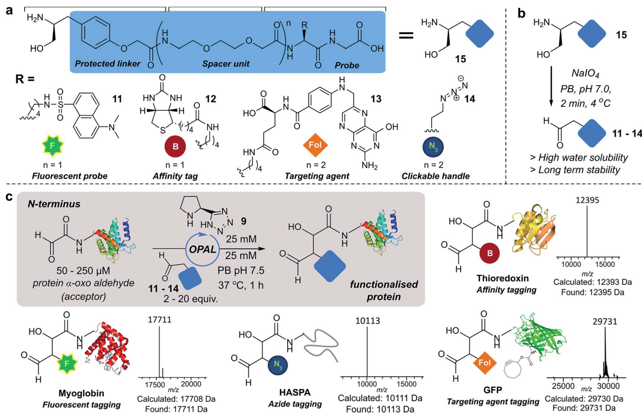
Fig. 3 (a) OPAL probe precursors bearing functional tags. (b) Mild \text{NaIO}_4 unmasking of α-aryl aldehyde probes. (c) OPAL functionalization of N-terminal α-oxo aldehyde containing proteins (50–250 μM), using probes 11–14 (0.5–1.5 mM).
