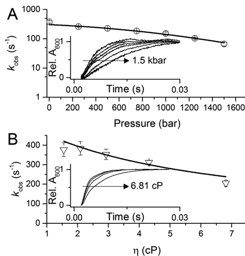
Fig. 3 The influence of (A) hydrostatic pressure and (B) solvent viscosity on PCET reactions catalysed by A \times NiR. The inserts in (A and B) show example transients for the pH-jump measurements used here to study PCET in A \times NiR. Data in (A and B) are fit to eqn (1) and (2), respectively.
