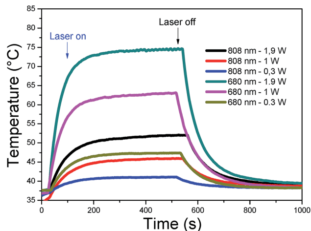
Fig. 6 Heating curves of CDs ( 40\text{ }\mu\text{g mL}^{-1} ) in PT mode under 808 and 680 nm laser (power: 0.3, 1, and 1.9\text{ W cm}^{-2} ).
