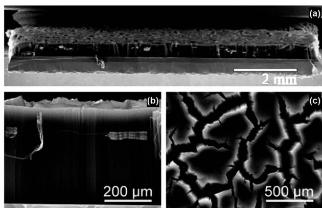
Fig. 8 FE-SEM images of a 420 μm thick SWCNT film on a 1 × 1 cm silicon wafer substrate prepared by microwave radiation: (a) the overview, (b) cross-sectional view and (c) top view. Reproduced from ref. 59, with permission from Wiley, 2005.
