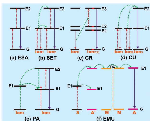
Fig. 3 Principal diagram for the upconversion processes of Ln 3+ -doped crystals. (a) ESA, (b) SET, (c) CR, (d) CU, (e) PA and (f) EMU. The red, green, and purple lines stand for photon excitation, energy transfer, and emission processes, respectively.
