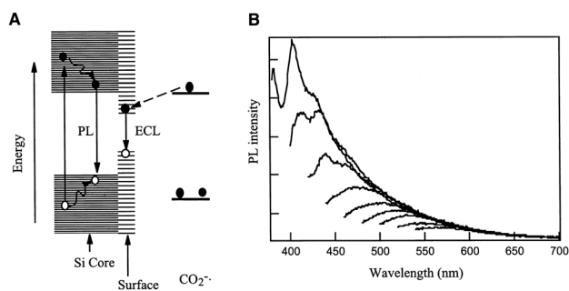
Fig. 3 (A) Schematic mechanisms for ECL and PL of Si clusters. (B) PL spectra at different excitation energies recorded with the same solution as in A. 60 Reprinted with permission from ref. 60. Copyright 2002 The American Association for the Advancement of Science.
