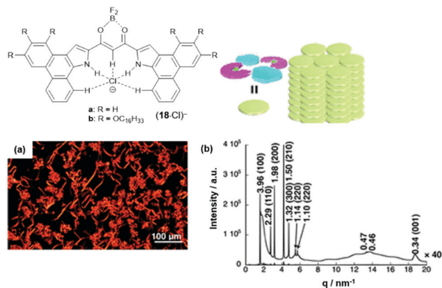
Fig. 18 Schematic representation of the phenanthro[b]-fused \pi -electronic anion ( 18\text{-Cl}^- ). (a) POM image of ( 14\text{a} )( 18\text{b-Cl} ) at 180\text{ }^\circ\text{C} upon cooling. (b) Synchrotron XRD pattern of ( 14\text{a} )( 18\text{b-Cl} ) at 150\text{ }^\circ\text{C} upon cooling; the proposed supramolecular packing mode of the assembly is also shown. 56 Figure reproduced with kind permission; © 2019 American Chemical Society.
