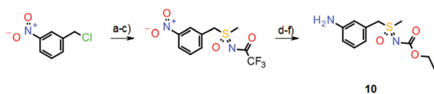
Scheme 6 Synthesis of key sulfoximine building block 10 in the initial preparation of atueveciclib. Reagents and conditions: (a) NaSMe, EtOH, -15^{\circ}\text{C} to rt, crude; (b) \text{H}_5\text{IO}_6 , \text{FeCl}_3 , MeCN, rt, 70%; (c) \text{CF}_3\text{C}(\text{O})\text{NH}_2 , \text{PhI}(\text{OAc})_2 , MgO, [\text{Rh}_2(\text{OAc})_4] , DCM, rt, 99%; (d) \text{K}_2\text{CO}_3 , MeOH, rt, 79%; (e) \text{ClC}(\text{O})\text{OEt} , pyridine, 0^{\circ}\text{C} to rt, crude; (f) \text{TiCl}_3 , THF, rt, crude.
