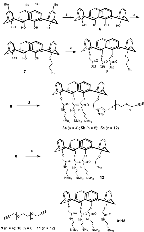
Scheme 2 Synthesis of targets 5a–c . Reaction conditions: (a) \text{AlCl}_3 , phenol, toluene, 98%; (b) 1-azido-2-iodoethane, \text{NaOMe} , \text{CH}_3\text{CN} , 85 °C, 67%; (c) ethyl bromoacetate, \text{K}_2\text{CO}_3 , \text{CH}_3\text{CN} , 85 °C; 65%; (d), (i) compound 9–11 , \text{CuI} , \text{CH}_3\text{CN} , 80 °C, microwave; (ii) N,N -dimethylethylenediamine, 50 °C, 10% in two steps ( 5a ), 23% in two steps ( 5b ), 27% in two steps ( 5c ); (e) N,N -dimethylethylenediamine, 50 °C, 39%.
