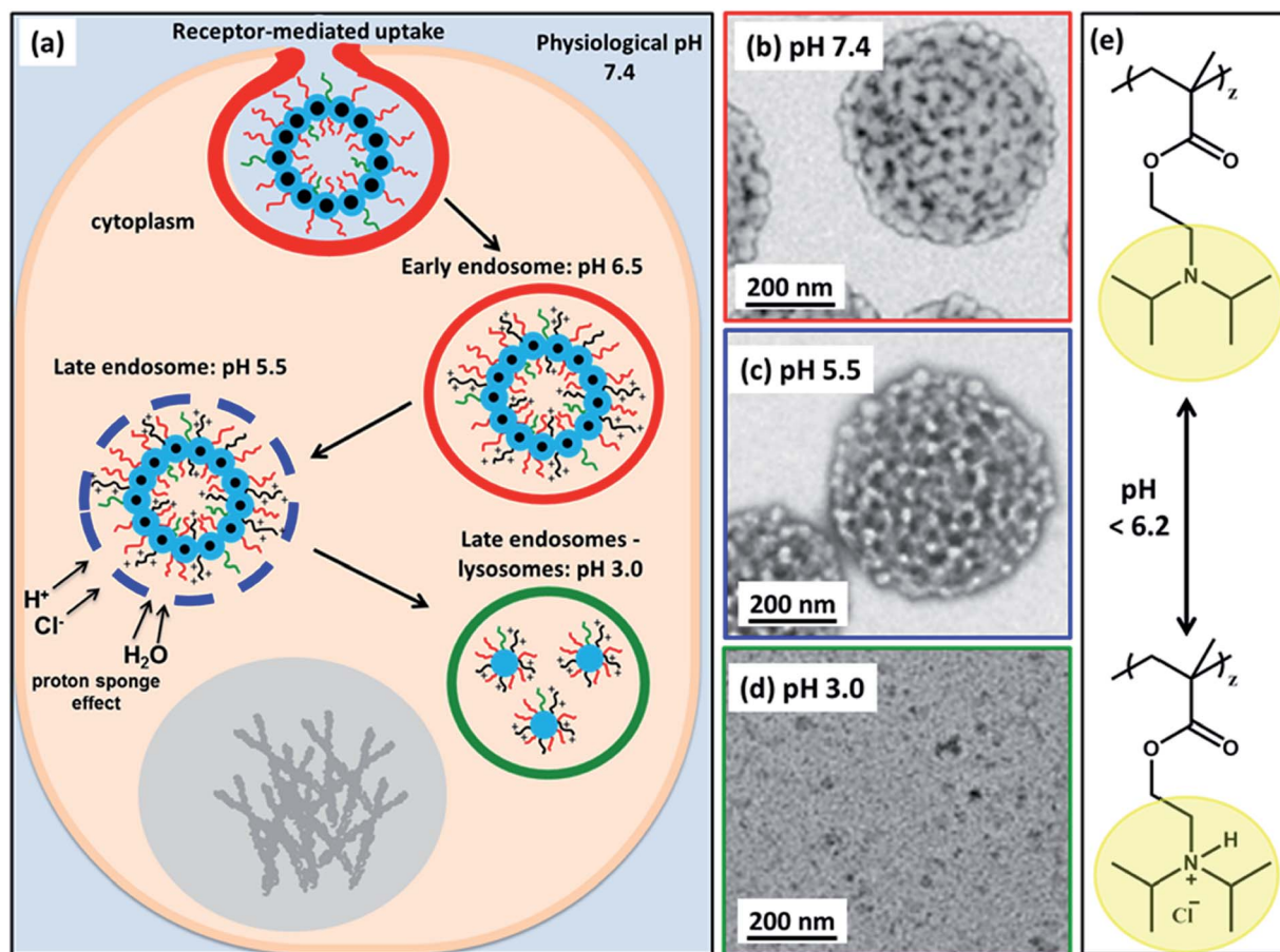
Fig. 7 (a) Schematic cartoon depicting the likely effect of intracellular acidification of (97 G_{58} + 3 M_{60})-(H_{300}\text{-stat-ERH}_1)\text{-D}_{52} nanoparticles during their endocytic internalization by MDA-MB-231 triple-negative breast cancer cells. After internalization by these cells, the vesicles are expected to remain intact at physiological pH, see TEM image (b). As the pH drops below pH 6.2 in the early endosomes, the PDPA block becomes partially protonated, see chemical structure shown in (e), and thus less hydrophobic, which leads to vesicle swelling (and perhaps greater porosity). At pH 5.5, the vesicle membrane becomes increasingly porous as the PDPA block loses its hydrophobic character, see TEM image (c). The gradual increase in cationic charge density is believed to trigger a 'proton sponge' effect 64 as water swells the late endosomes to counteract the increase in ionic strength. This should cause temporary rupture of the endosomes and release of its cargo into the nuclear region. 64,65 In the lysosomes the local pH is 3.0. The PDPA block is expected to be fully protonated at this pH, leading to the formation of weakly-interacting cationic spherical micelles, see TEM image (d). These pH-induced morphological transitions can be studied by TEM for dilute aqueous vesicle dispersions dried at (b) pH 7.4, (c) pH 5.5 and (d) pH 3.0. (e) Chemical structure of the PDPA block when fully deprotonated above pH 6.2 and when full protonated below pH 6.2 (this pH approximately corresponds to the pK_a of the PDPA block, although this parameter is dependent on the ionic strength).
