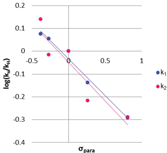
Fig. 5 Hammett plots for the two individual rate constants for the 2\text{Ph-X} derivatives. Trendlines for k_1 ( y = -0.32x - 0.033 ) and k_2 ( y = -0.34x - 0.047 ) are shown.
