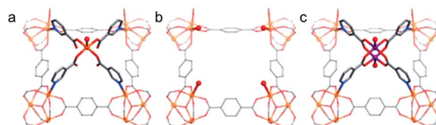
Fig. 11 Key local structures of (a) MCF-37, (b) the [Fe 3 (μ 3 -O)(BDC) 3 (L T ) 3 ] scaffold, (c) MCF-49. Color code: C, gray; O, red; N, blue; Fe, orange; and Co, purple. H atoms are omitted for clarity. Adapted from ref. 180 with permission from the American Chemical Society, copyright 2017.
