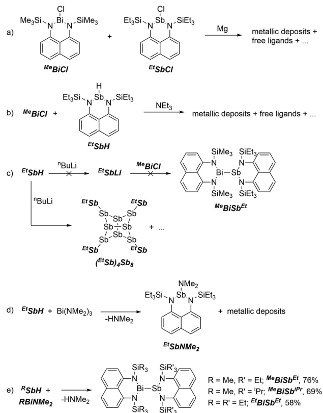
Scheme 2 Synthesis of ( EtSb ) 4 Sb 8 and derivatives of R i BiSb R' .
