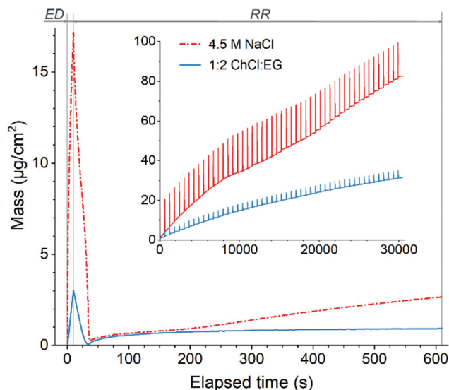
Fig. 2 Variation of mass during one EDRR cycle (10 s ED + 600 s RR) in aqueous 4.5 M NaCl solution and 1 : 2 ChCl : EG (60 mM Cu, 0.5 mM Au, T = 25^\circ\text{C} ). Inset: mass change throughout 50 EDRR cycles.
