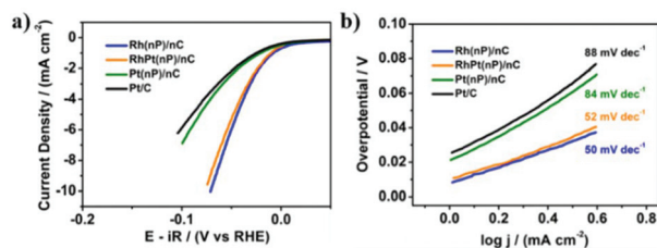
Fig. 3 HER performance of Rh(nP)/nC, RhPt(nP)/nC, Pt(nP)/nC and commercial Pt/C in 0.1 M KOH solution. (a) LSV polarization curves at a scan rate 5 mV s -1 . (b) Corresponding Tafel plots. The potentials were corrected for iR drop and calibrated to RHE.
