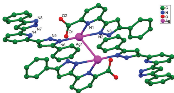
Fig. 34 The molecular structure showing the ligand-unsupported argentophilic interactions in 56 .
