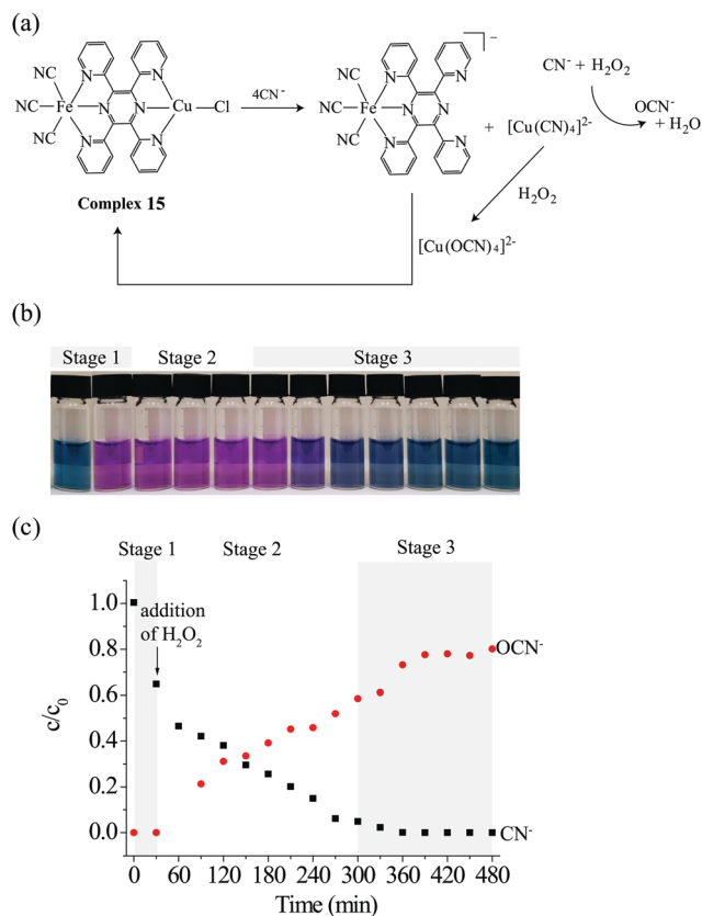
Fig. 9 Reversible detection of cyanide by 15 via the degradation of newly formed “receptor–cyanide ensemble”, i.e. [Cu I (CN) 4 ] 2- , under the ICDA.
