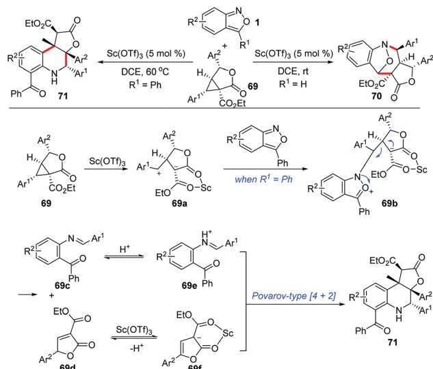
Scheme 25 Sc(OTf) 3 -Catalysed chemodivergent annulations of γ-butyrolactone-fused cyclopropanes with anthranils.
