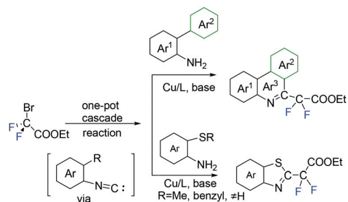
Scheme 110 The reaction of \text{BrCF}_2\text{COOEt} with primary amines.
