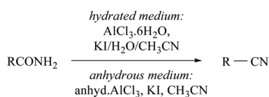
Scheme 4 AlCl 3 as a dehydrating agent.
