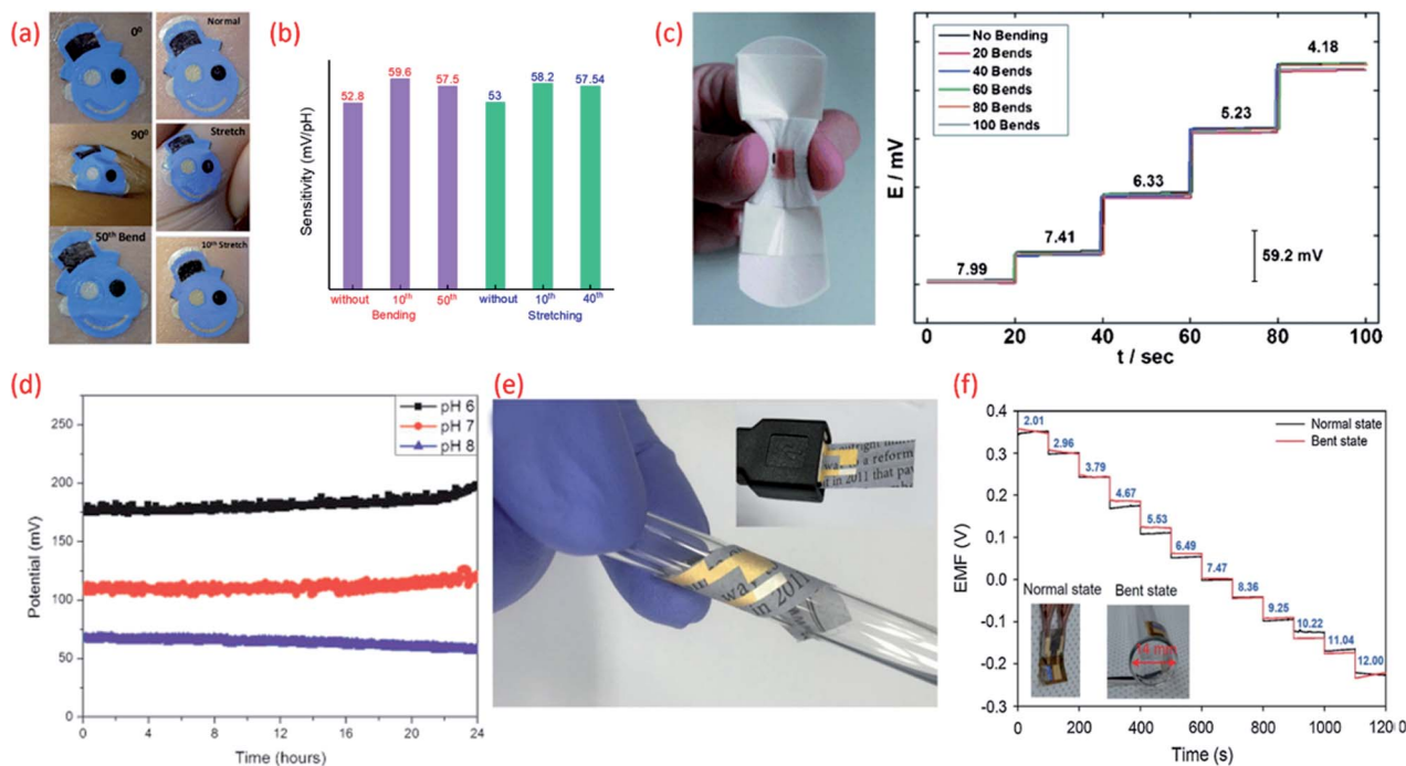
Fig. 5 (a) Images of the tattoo pH sensor with PANi sensitive electrode applied to cubital fossa at 0° bending, 90° bending, and after the 50 th bending and Images at normal, during stretching, and after the 10 th stretch Reprinted with permission from Publication. 210 (b) The comparison of sensitivity variation of the tattoo-based sensors under different bending stretching condition Reprinted with permission from Publication. 210 (c) Image of bandage-based pH sensor with PANi electrode in bending condition and its calibration curves from pH 7.99 to 4.18 (each trace taken after 20 bends) Reprinted with permission from John Wiley and Sons. 152 (d) Long-term potential stability of the wound monitoring pH sensors (based on PANi electrode) at pH 6, pH 7 and pH 8 (pH values observed during chronic wound healing) Reprinted from Publication 206 with permission from Elsevier. (e) Image of USB-type sensing platforms and flexible state of ion-selective sensor Reprinted from Publication 134 with permission from Elsevier. (f) Response of pH sensors (PANi electrode) with increasing pH levels under mechanically normal and bent states (image shown in inset) Reprinted from Publication 134 with permission from Elsevier.
