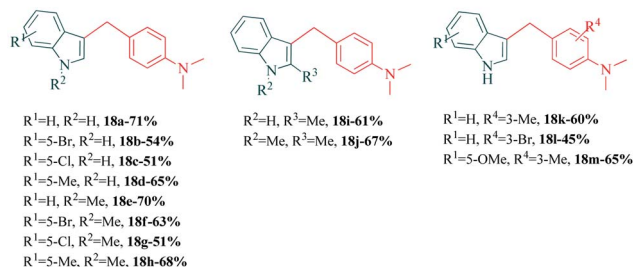
Scheme 5 Visible light promoted synthesis of C3-alkylated indoles.
