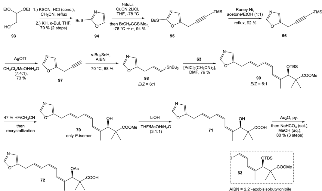
Scheme 7 Synthesis of the left-hand fragment derivative 72 of neoxazolomycin by Hatakeyama.
