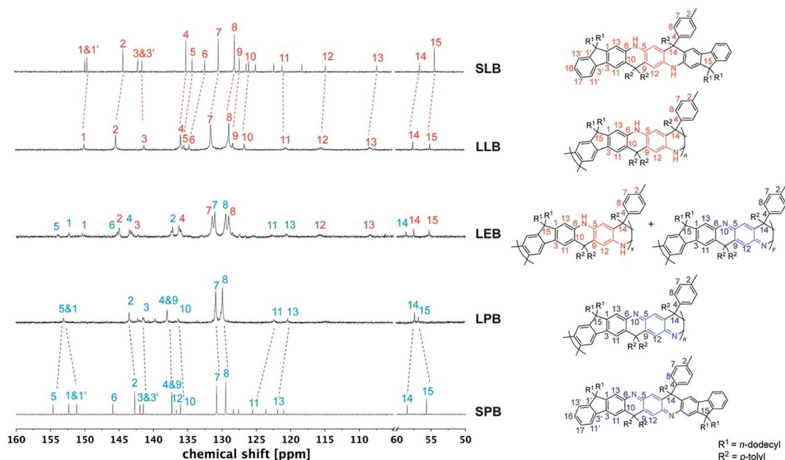
Fig. 2 ^{13}\text{C} NMR spectra of small molecule model SLB and SPB, and varied oxidation states of LPANI ( d_8\text{-THF} at 298 K).
