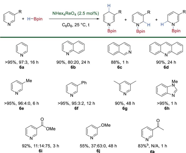
Scheme 5 Catalytic hydroboration of N-heteroaromatics using [\text{N}(\text{hexyl})_4][\text{ReO}_4] as a pre-catalyst and HBpin. For 6k reduction is observed exclusively at the carbonyl when 1 equivalent of HBpin is used.
