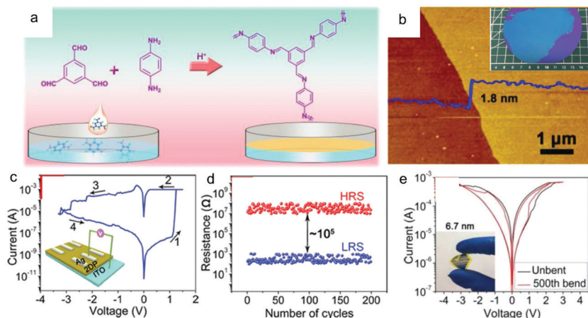
Fig. 16 (a) A schematic illustration of the synthesis of 2DP_{BTA+PDA} films through the Schiff-base reaction of the monomers. (b) AFM image of a 1.8 \pm 0.2 nm thick 2DP_{BTA+PDA} film on a silicon wafer. (c) I - V plots for the initial formation process (inset: the schematic diagram of the resistive switching device with a Ag/ 2DP_{BTA+PDA} /ITO configuration). (d) Endurance performance of the on/off resistances plotted as a function of the number of cycles. (e) Switching curves of a flexible Ag/ 2DP_{BTA+PDA} /graphene device before and after repeated mechanical bending of up to 500 cycles (inset: a photograph of the flexible device under bending). Reproduced with permission from ref. 175. Copyright 2019 Wiley & Sons.
