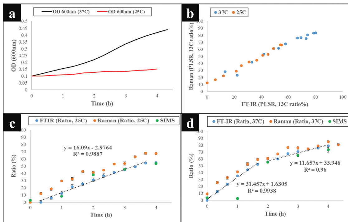
Fig. 3 (a) Growth profiles ( \text{OD}_{600} ) of E. coli grown in minimal medium at 37 and 25 °C, illustrating higher optical density for cells grown at 37 °C than cells cultivated at 25 °C. (b) Plot of FT-IR vs. Raman PLSR predicted ^{13}\text{C} content of the cells, indicating the results are in agreement. Predicted levels of ^{13}\text{C} content in cells using the shift in amide I band upon incorporation of ^{13}\text{C} by cells ( 1616/1654\text{ cm}^{-1} for FT-IR spectra and 1622/1661\text{ cm}^{-1} for Raman spectra) and m/z of 16 ( ^{13}\text{CH}_3 ) and 15 ( ^{12}\text{CH}_3 ) ( ^{13}\text{CH}_3/^{12}\text{CH}_3 + ^{13}\text{CH}_3 ) for SIMS spectra) at (c) 25 and (d) 37 °C growth temperatures.
