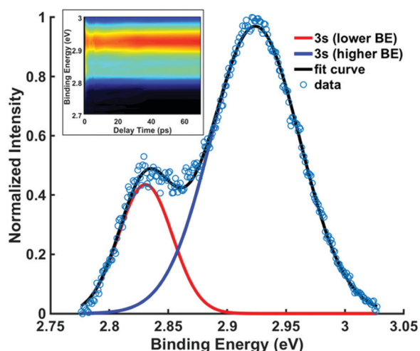
Fig. 6 The normalized intensities of the overlapping 3s component peaks (229 nm excitation) after equilibrium is reached, with delay times between 6 ps and 70 ps. The data (blue circles) are fitted with two Gaussian functions (blue and red curves) centered at 2.83 eV and 2.92 eV. The inset shows two 3s state peaks up to 70 ps in 229 nm excitation spectrum.
