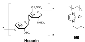
Fig. 19 Structure of 160 and heparin.
