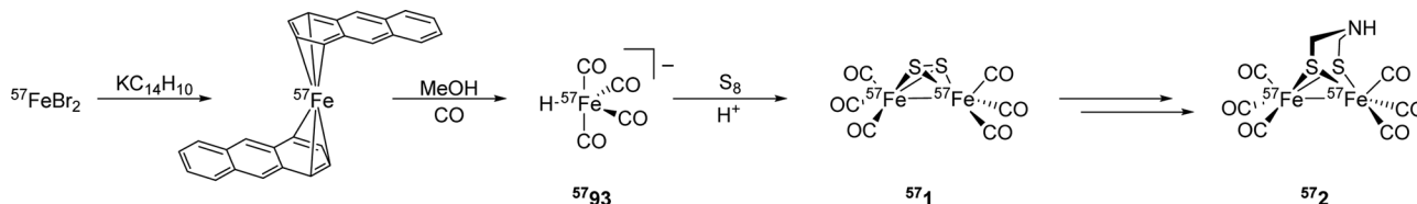
Fig. 33 Synthetic pathway to ^{57}Fe_2(adT)(CO)_6 .
