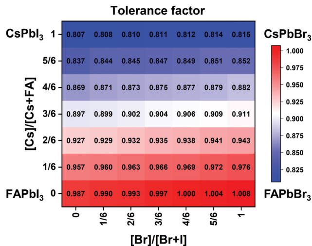
Fig. 2 Effective tolerance factor map for the \text{Cs}_x\text{FA}_{1-x}\text{Pb}(\text{Br})_y\text{I}_{1-y} compositional space tuned via composition engineering.
