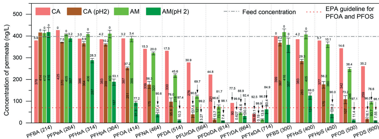
Fig. 1 Concentrations of PFCAs and PFSAs in the permealte. The pH of the feed is around 7 unless otherwise stated. The number in the brackets is the MW of each compound. The red dashed line stands for EPA guideline for PFOA and PFOS regulation, which is 70 \text{ ng L}^{-1} . The grey dashed line stands for the spike concentration of each PFAS, which is around 400 \text{ ng L}^{-1} . The removal efficiencies (%) are shown above the permealte bars.
